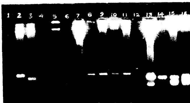
Figure 1. PCR amplification of clinical samples using TRC4 and IS6110 primers. Lane 1, Negative control (no DNA) with TRC4 primers; Lane 2, positive control ( M. tuberculosis H 37 Rv DNA) with TRC4 primers amplifying 173 bp product; Lane 3, positive control ( M. tuberculosis H 37 Rv DNA) with IS6110 primers amplifying 123 bp product; Lane 4, negative control (no DNA) with IS6110 primers; Lane 5, molecular weight marker ( Hind III); Lane 6, processing control with TRC4 primers (water blank included during of the clinical sample); Lane 7, a negative clinical sample (with TRC4 primers); Lanes 8 to 11, clinical samples which show 173 bp; Lane 12, processing control with IS6110 primers (water blank included during processing of the clinical sample); Lanes 13 to 16, positive clinical samples which show 123 bp product.
